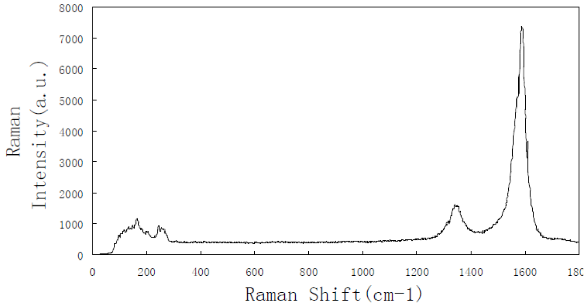
Raman Spectrum of SWCNTs
